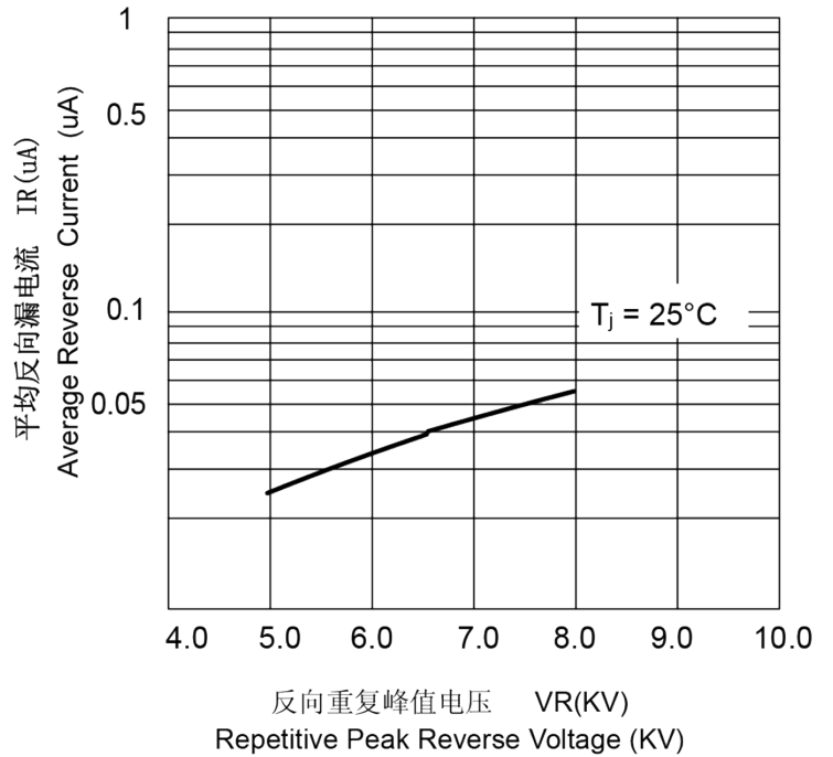
REVERSE CHARACTERISTIC [VR-IR]
