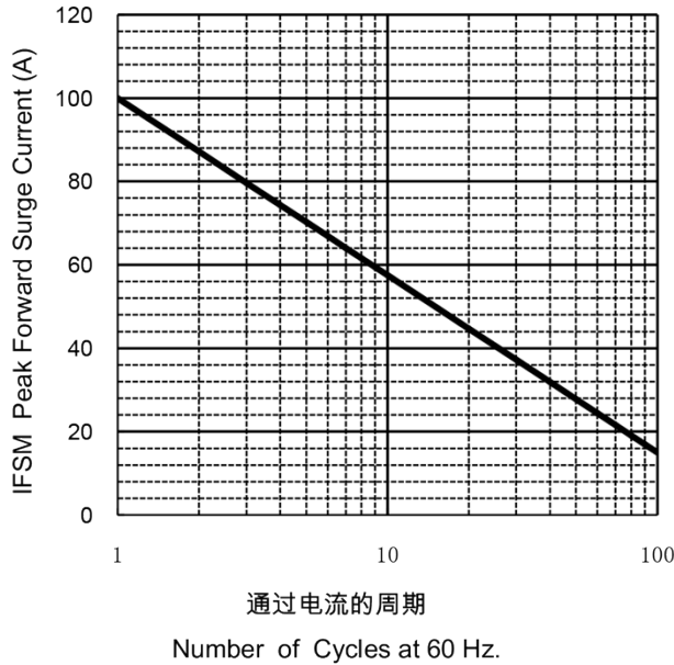
PEAK FORWARD SURGE CURRENT
